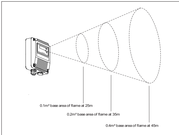
Fig 1 Flame detection as a function of flame size and distance from detector
